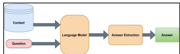
Fig. 2 Answer Extraction[19]
